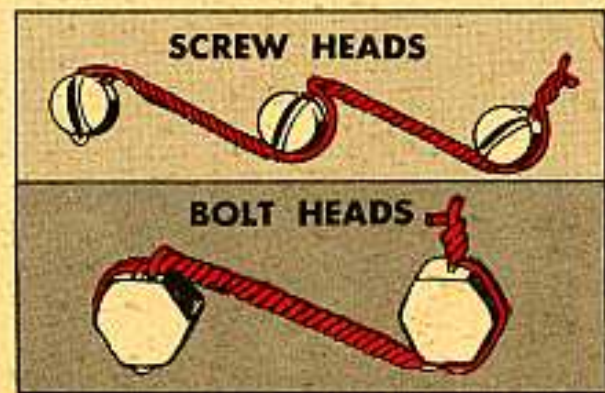
In the two cases above the safety wire goes over the head while in the two cases below the safety wire goes around the head. Safety methods shown are for right hand threads—left hand opposite.
