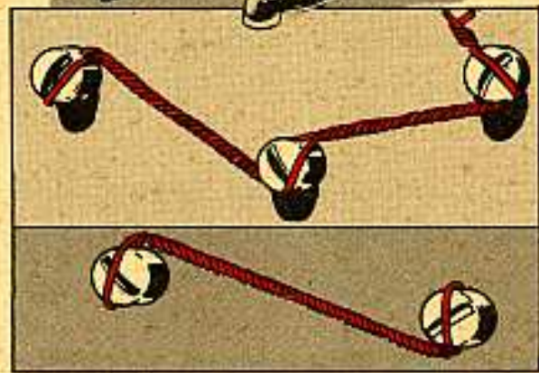
In the two cases above the safety wire goes over the head while in the two cases below the safety wire goes around the head. Safety methods shown are for right hand threads—left hand opposite.
