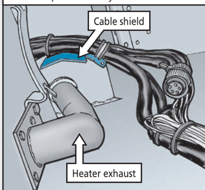
Shield keeps cables away from heater exhaust
