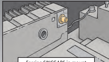
Forcing SINGGARS in mount damages P1 and GPS connectors
