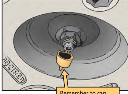
Clean recessed area and give fitting four to five shots of grease
