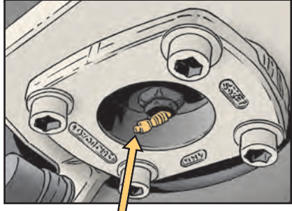
Clean recessed area and give fitting four to five shots of grease
